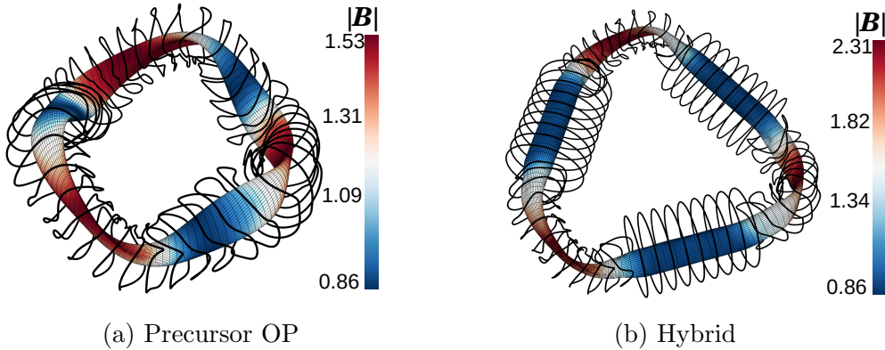
Figure A1: An n_{\text{FP}} = 3 precursor OP in figure A1a calculated in DESC and a corresponding stellarator-mirror hybrid in figure A1b calculated in GVEC . The choice of mirror coil current causes the mirror ratio B_{\text{max}}/B_{\text{min}} to differ from the precursor OP equilibrium.
