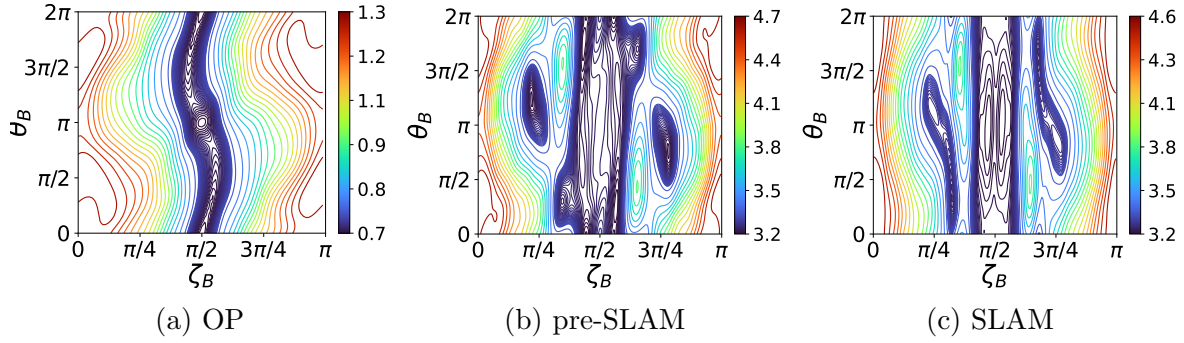
Figure 7: Magnetic field strength in Boozer coordinates for the precursor OP, pre-SLAM, and SLAM equilibria on their respective boundaries. The mirror region lies in low-field region. Using an axisymmetrized mirror brings the low field region closer to a QuasiPoloidal configuration by closing or straightening more puddles and making more |\mathbf{B}| contours closed in \theta_B compared to the pre-SLAM case.
