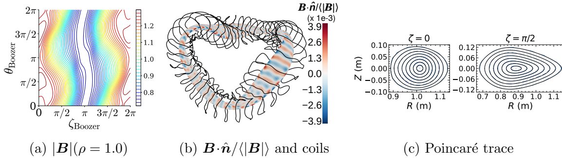
Figure 1: A n_{\text{FP}} = 2 vacuum OP equilibrium and its corresponding coilset from the DESC omnigenity database [39]. Figure 1a represents the field strength in Boozer coordinates. In Figure 1b plots the OP coilset and the normalized field error \mathbf{B} \cdot \hat{\mathbf{n}} / \langle |\mathbf{B}| \rangle on the equilibrium boundary, where \langle \rangle is a surface average. Figure 1c traces the field lines from the coils and compares them with equilibrium flux surfaces. The coilset field-line trace matches well with the flux surfaces.
