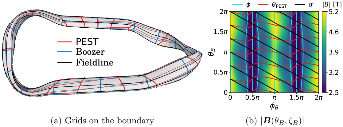
Figure 5: In figure 5a, we present a pre-SLAM surface mapped using the FTGen algorithm showing grids corresponding to different coordinate systems. Contours of constant \zeta_B result in a cross-section that is approximately normal to the mirror region whereas contours of constant cylindrical angle lead to an oblique cross-section. In figure 5b, we plot the |B| on the surface in Boozer coordinates and contours of constant PEST coordinates and the fieldline label \alpha .
