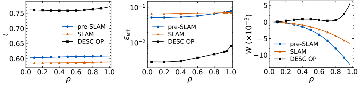
Figure 8: Comparison of the rotational transform, effective ripple, and the magnetic well between the original OP, pre-SLAM, and SLAM equilibria. Both the ripple and magnetic well are worse after converting the OP coilset into a stellarator-mirror hybrid coilset. The SLAM ripple is worse in the core but better in the edge, and its magnetic well is better than that of the corresponding pre-SLAM.
