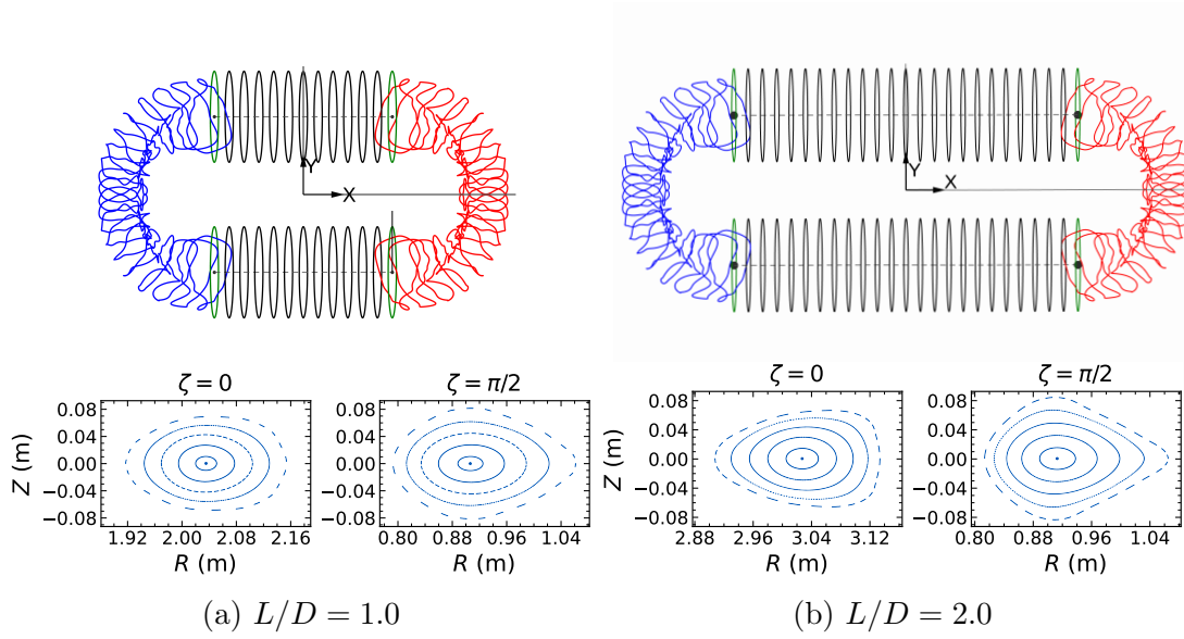
Figure 3: Stellarator-mirror hybrid coilset using the OP coilset presented in figure 1b with two different mirror lengths and their corresponding Poincaré plots on the planes where the black lines intersect the coils. Nested surfaces exist even after separating the OP coilset and adding mirror coils. Note that the cross-section in the mirror is not a circle (axisymmetric).
