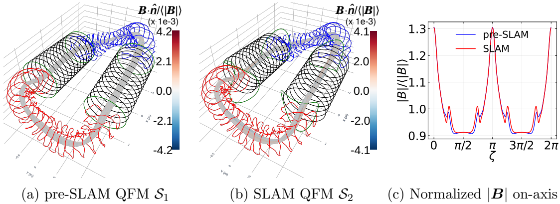
Figure 4: The pre-SLAM and SLAM coilsets and QFM surfaces along with the magnetic field on axis for the two coilsets. Note that only a single unique converter coil is changed. The converter coil increases the magnetic field ripple in the converter region around \zeta = \pi/4, 3\pi/4, 5\pi/4, 7\pi/4 as shown in figure 4c, while axisymmetrizing the mirror and keeping the stellarator boundary almost exactly the same. As a consequence, the |B| in the stellarator region is identical for both the pre-SLAM and SLAM coilsets.
