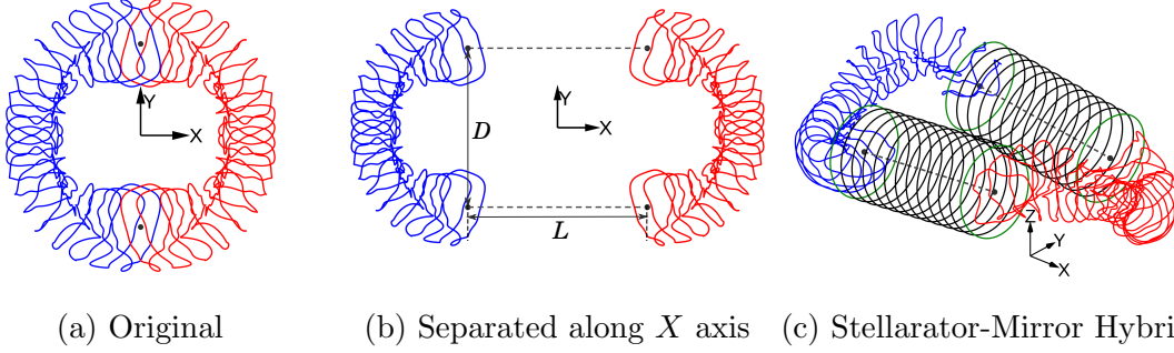
Figure 2: Process of making a stellarator-mirror hybrid coilset. We start with the original OP coilset in figure 2a, separate it at the point of lowest magnetic field strength and vanishing axis curvature, along the X axis by a distance L in figure 2b, and using the (dashed) line joining the magnetic axis in the original coilset as the center, place circular mirror coils in the gap as shown in figure 2c.
