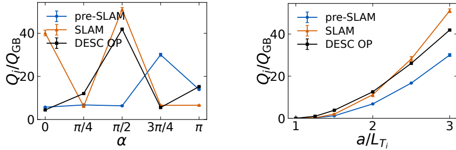
Figure 9: Nonlinear ITG heat flux Q from GX for the original OP, pre-SLAM, and SLAM equilibria at \rho = 0.8 . Left: Q as a function of the field-line label \alpha at a normalized ion-temperature gradient a/L_T = 3 . Right: Q as a function of a/L_T on the field line with the largest heat flux.
