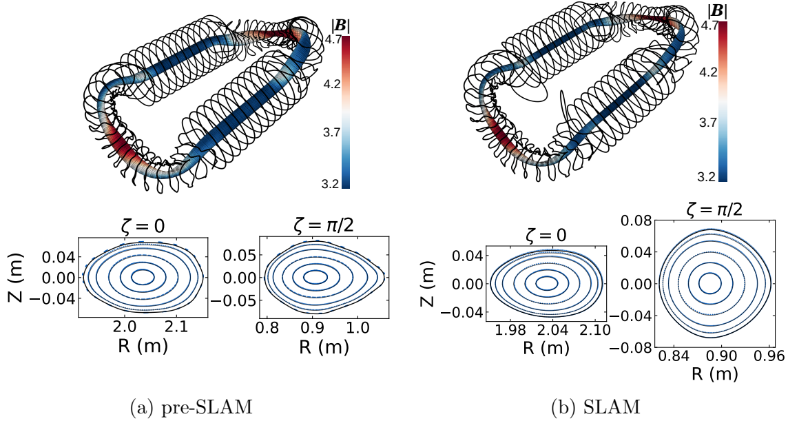
Figure 6: Comparison of the fixed-boundary GVEC solution with the Poincaré trace from the coilset, demonstrating an excellent match between the GVEC surfaces and the Poincaré data. Note that, even though the surfaces are nested at larger radii, the SLAM equilibrium was truncated to a smaller radius because the outer surfaces become non-circular in the mirror region, making the SLAM equilibrium smaller.
