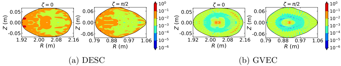
Figure B1: Comparison of the normalized force balance error at two different cross-sections obtained by solving the equilibrium for the pre-SLAM boundary corresponding to \mathcal{S}_1 in figure 4a. The boundary data was calculated by tracing the field line using the FTGen algorithm and fed to both codes. The DESC case solved the equilibrium problem in native DESC coordinates whereas GVEC solved the problem in generalized coordinates.
